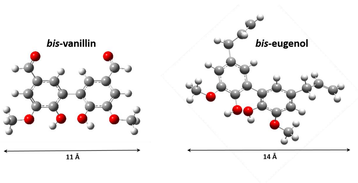
Figure 1. Optimized geometries of bis-vanillin and bis-eugenol.
