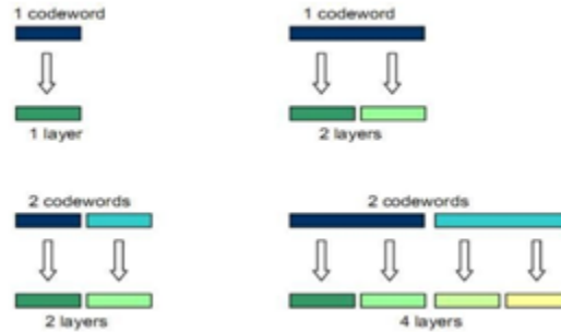
Fig. 7 layer mapping for spatial multiplexing.
