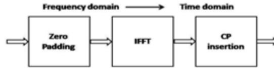
Fig. 9 The structure of OFDM modulation
