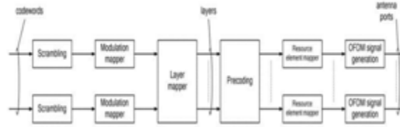
Fig. 5 Overview of physical channel processing
