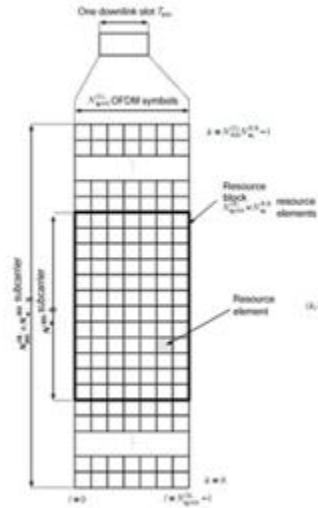
Fig. 8 Downlink resource grid
