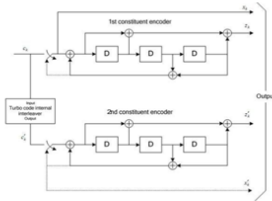
Fig. 4 Structure of rate 1/3 turbo encoder (dotted lines apply for trellis termination only).
