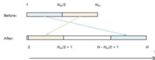
Fig. 10 Zero padding of OFDM modulation.
