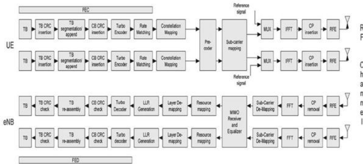
Fig. 2 Downlink PHY block diagram [8].
