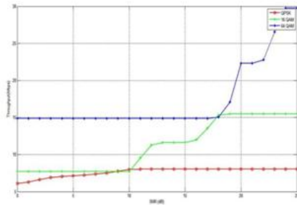
Fig. 18 4X4 MIMO Downlink Throughput in 5 MHz bandwidth.
